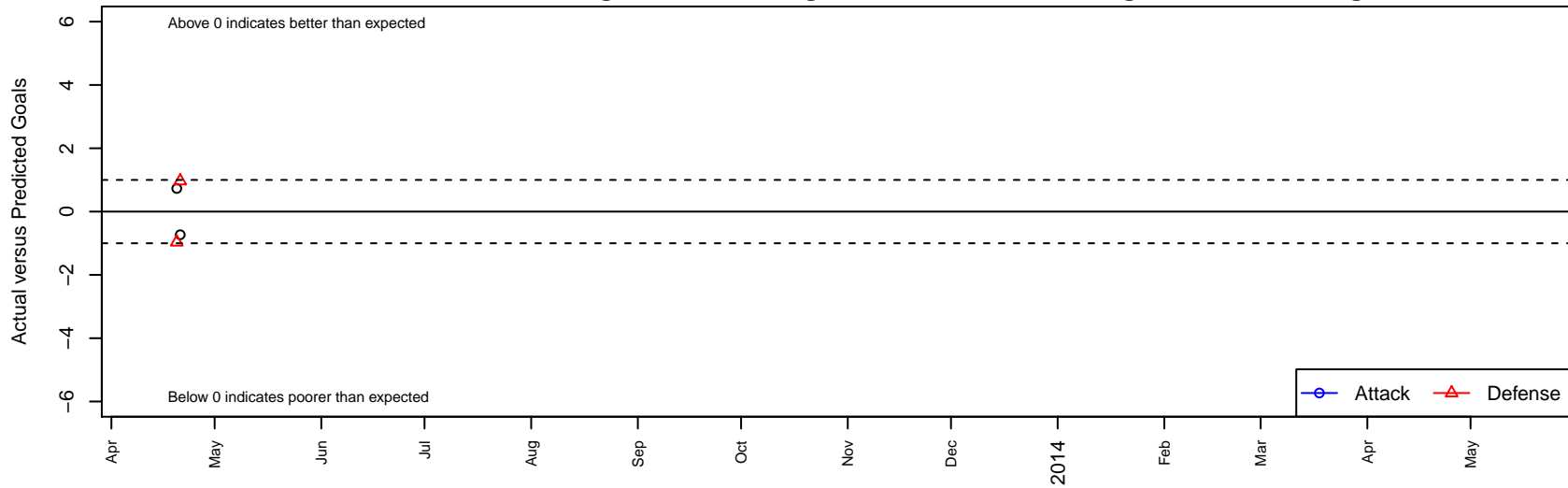
THUSC Iron B99 Dots are actual minus expected GF (blue circles) and GA (red triangles). Blue line is smoothed change in attack strength. Red is smoothed change in defense strength.
